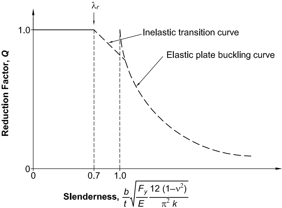
Fig. C-E7.1. Definition of Q_s for unstiffened slender elements.
