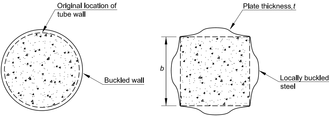
Fig. C-I1.2. Change in cross-sectional buckling mode due to concrete infill.
