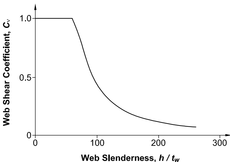
Fig. C-G2.1. Shear buckling coefficient C_v for F_y = 50 \text{ ksi (345 MPa)} and k_v = 5.0 .
