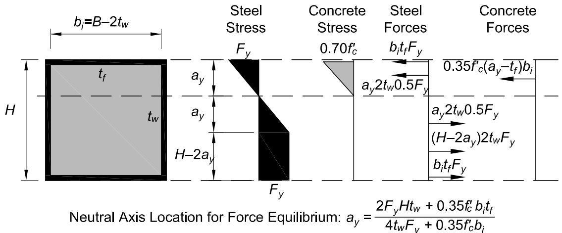
(b) Noncompact section—stress blocks for calculating M_y
