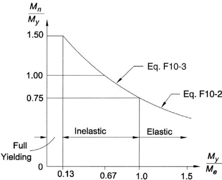
Fig. C-F10.1. Lateral-torsional buckling limits of a single-angle beam.
