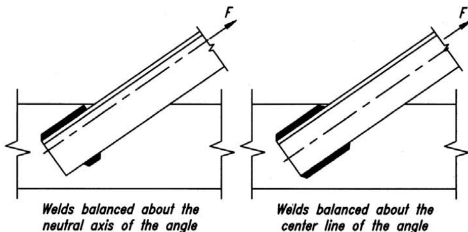
Fig. C-J1.3. Balanced welds
