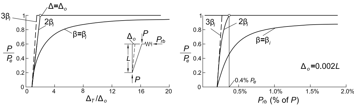
Fig. C-A-6.3. Effect of initial out-of-plumbness.
