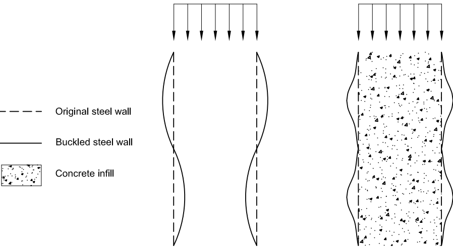
Fig. C-I1.3. Changes in buckling mode with length due to the presence of infill.
