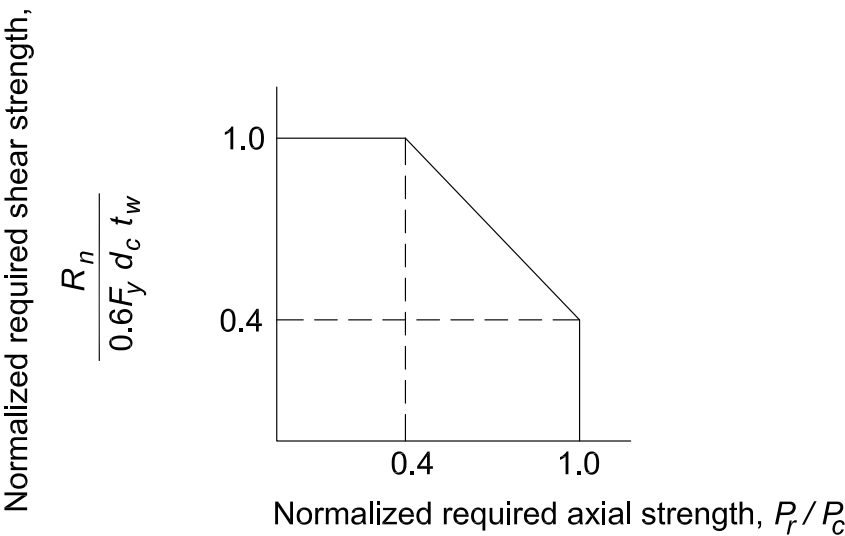
Fig. C-J10.4. Interaction of shear and axial force—elastic.
