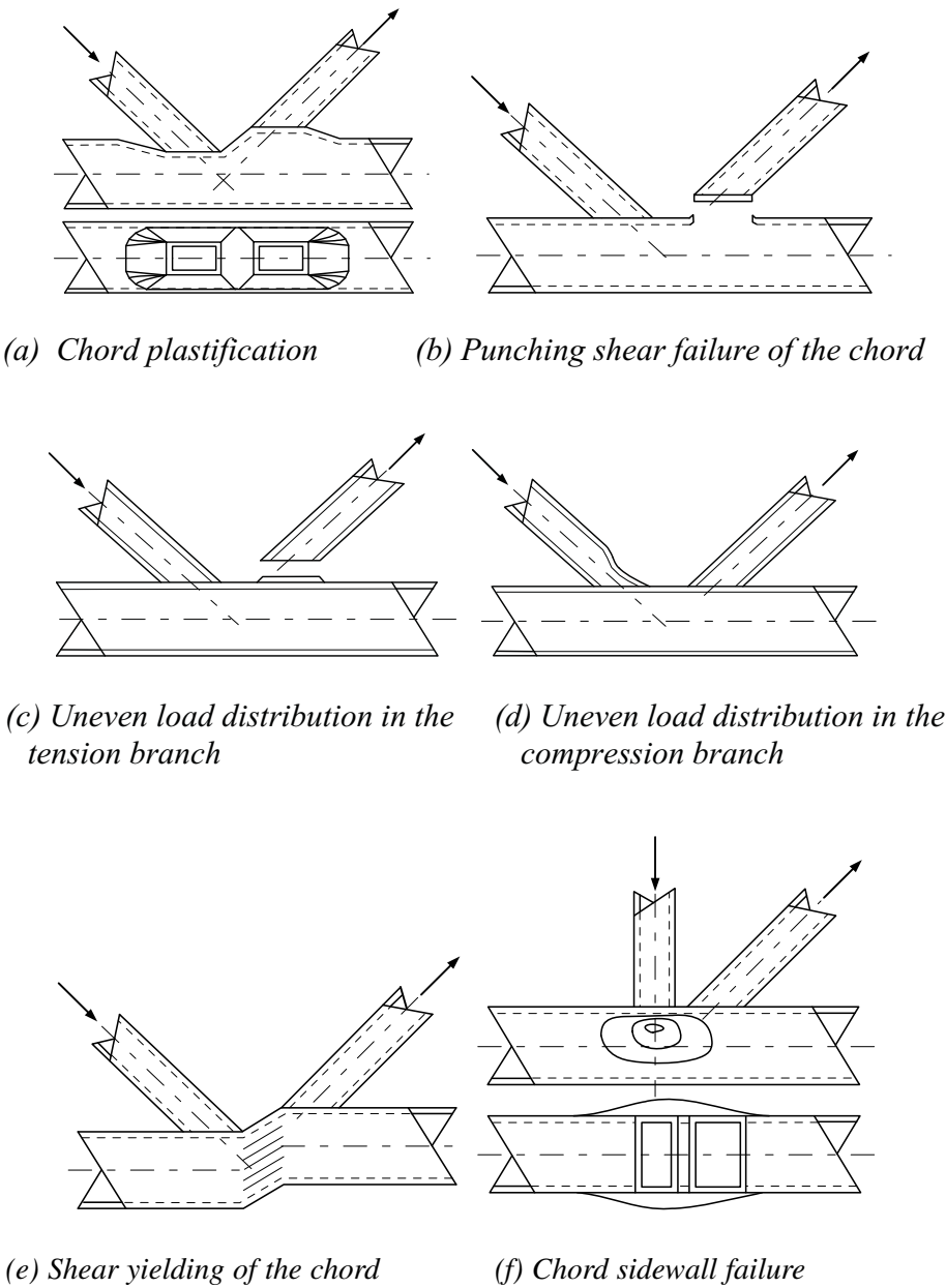
Fig. C-K2.3. Typical limit states for HSS-to-HSS truss connections.
