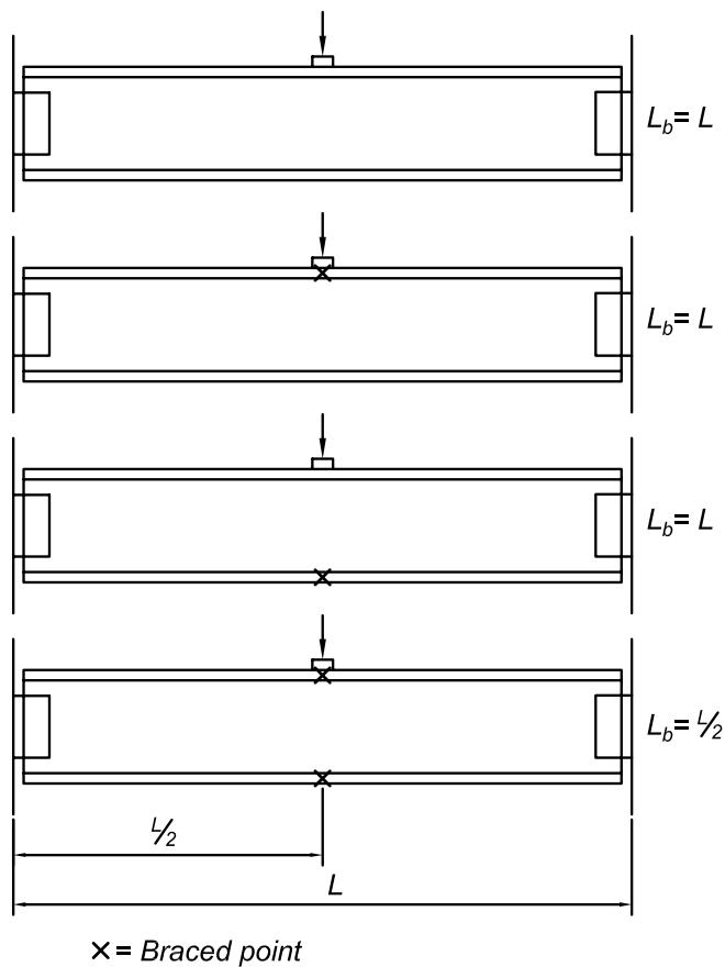
Fig. C-J10.2. Unbraced flange length for web sidesway buckling.
