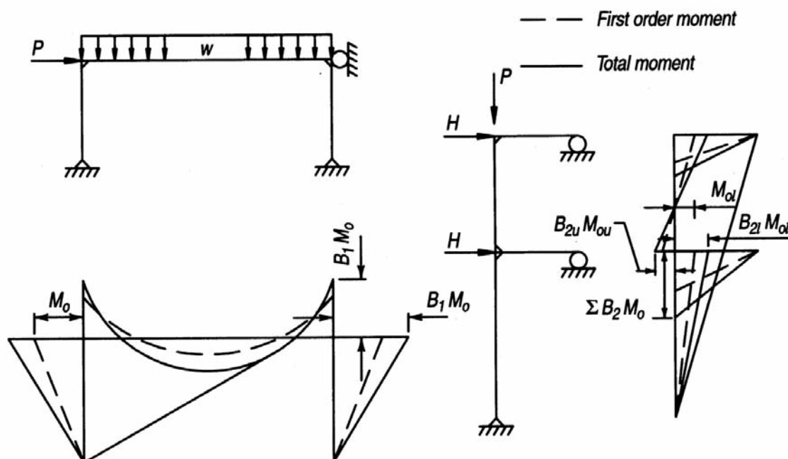
Fig. C-A-8.1. Moment amplification.
