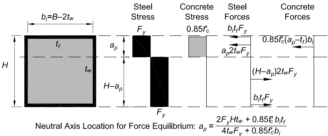
(a) Compact section—stress blocks for calculating M_p
